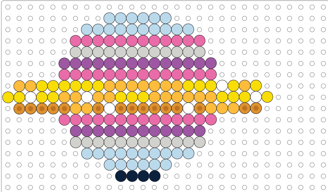
Saturn
